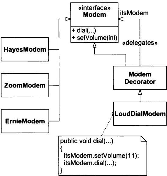
Figure 28-6 ModemDecorator
