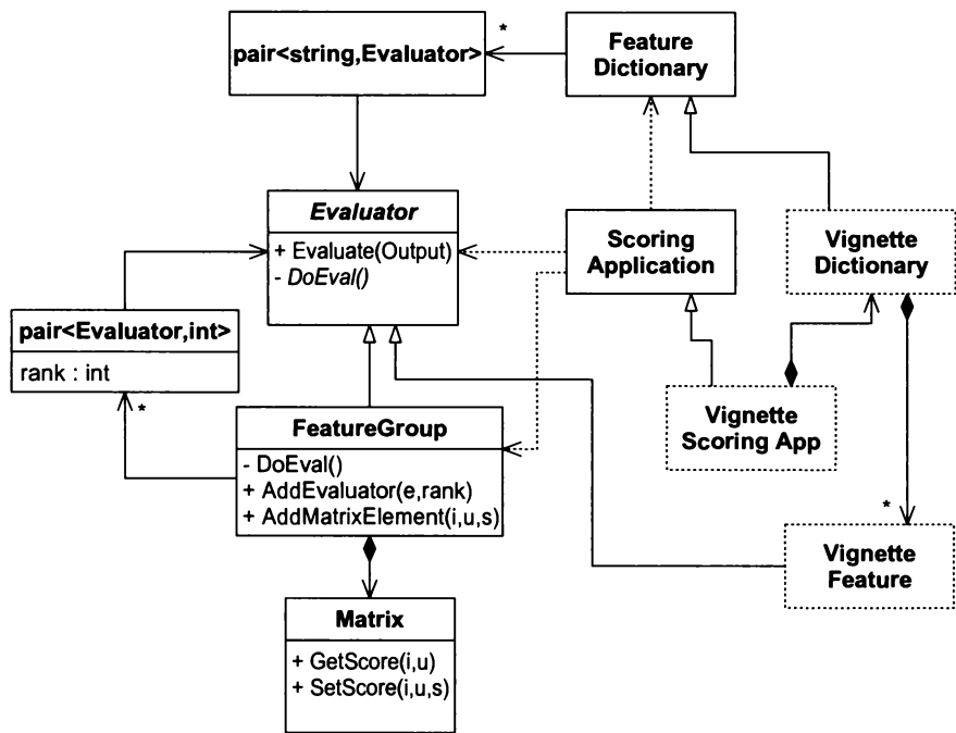
Figure 30-3 Scoring Framework
