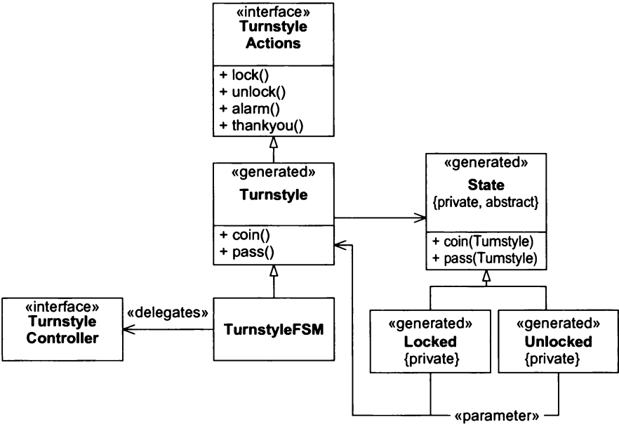
Figure 29-5 Three-Level FSM
